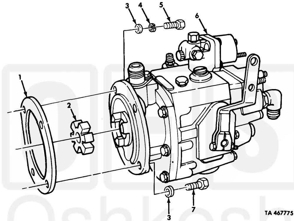
Figure 28. Fuel Pump Assembly, AFC.
